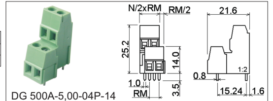
DG 500A-5,00-04P-14
