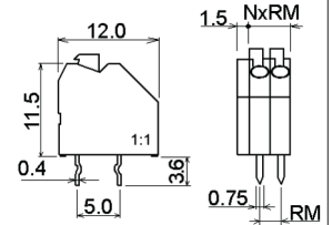
DG250-2.50-02P-11
