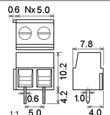
DG126-5,00-03P-14
