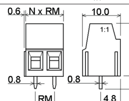
DG500-5,00-03P-14
