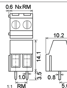
DG128-5,00-03P-14
