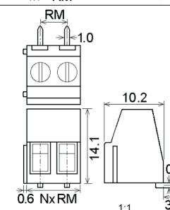
DG128R-5,00-03P-14
